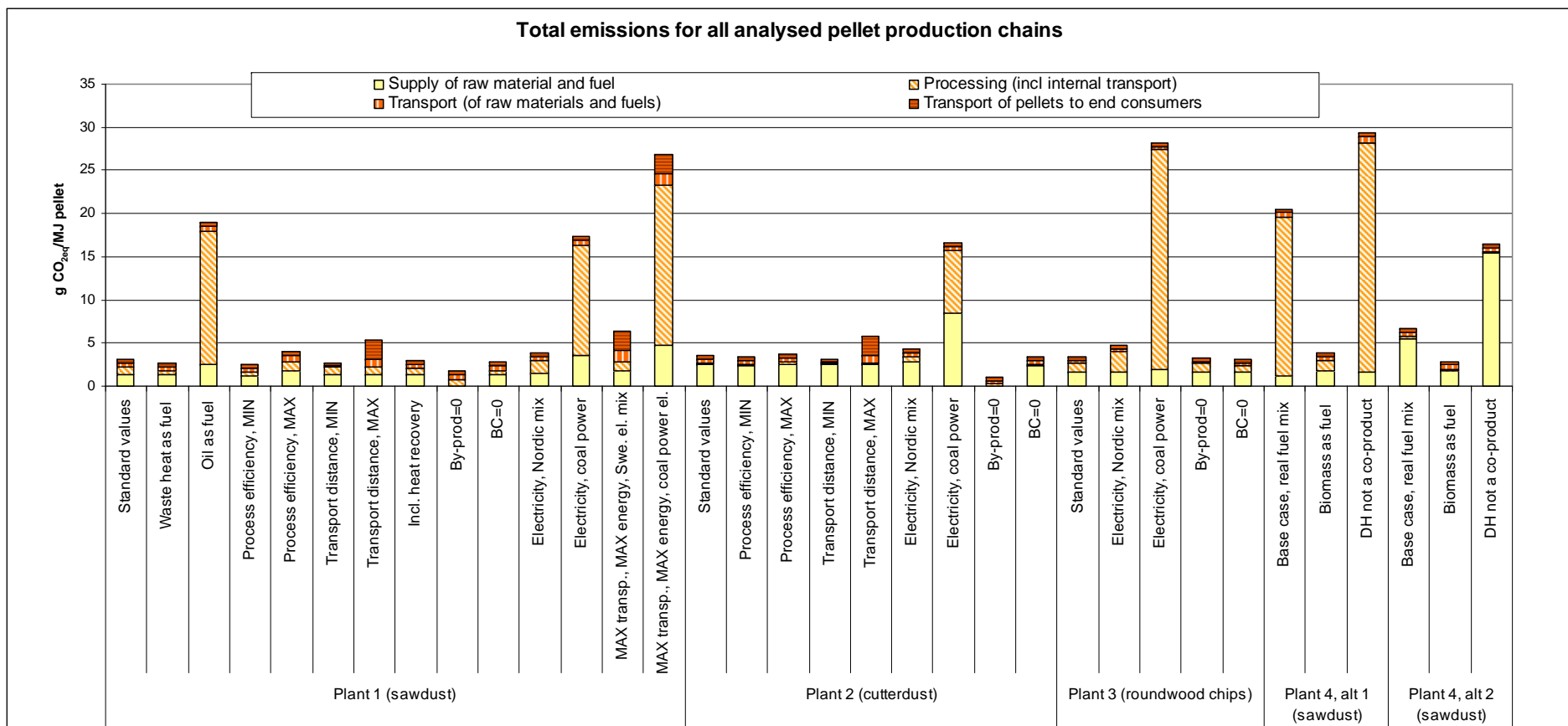
Figure S1 Summary of results for the different pellet production chains analysed. Plant 1-3 indicate production in stand-alone pellet plants. Plant 4 is production in a pellet plant integrated with a CHP plant (Hedensbyn) where alt 1) it is regarded as a poly-generation plant, and alt 2) the pellet plant and the CHP are regarded as separate plants. The following assumptions are used, if not otherwise stated: Swedish electricity mix; typical values for process efficiency (energy) and transport distances; emissions from production of saw mill by-products and biomass combustion are accounted for; biomass used for drying in Plant 1 and Plant 3; for Plant 4 the fuel mix in the CHP is 26% peat and 74% biomass and district heating is regarded as a co-product. Explanations: By-prod=0 when emissions from saw mill by-products are taken as zero; BC=0 when all emissions from biomass combustion is taken as zero. DH means district heating.
