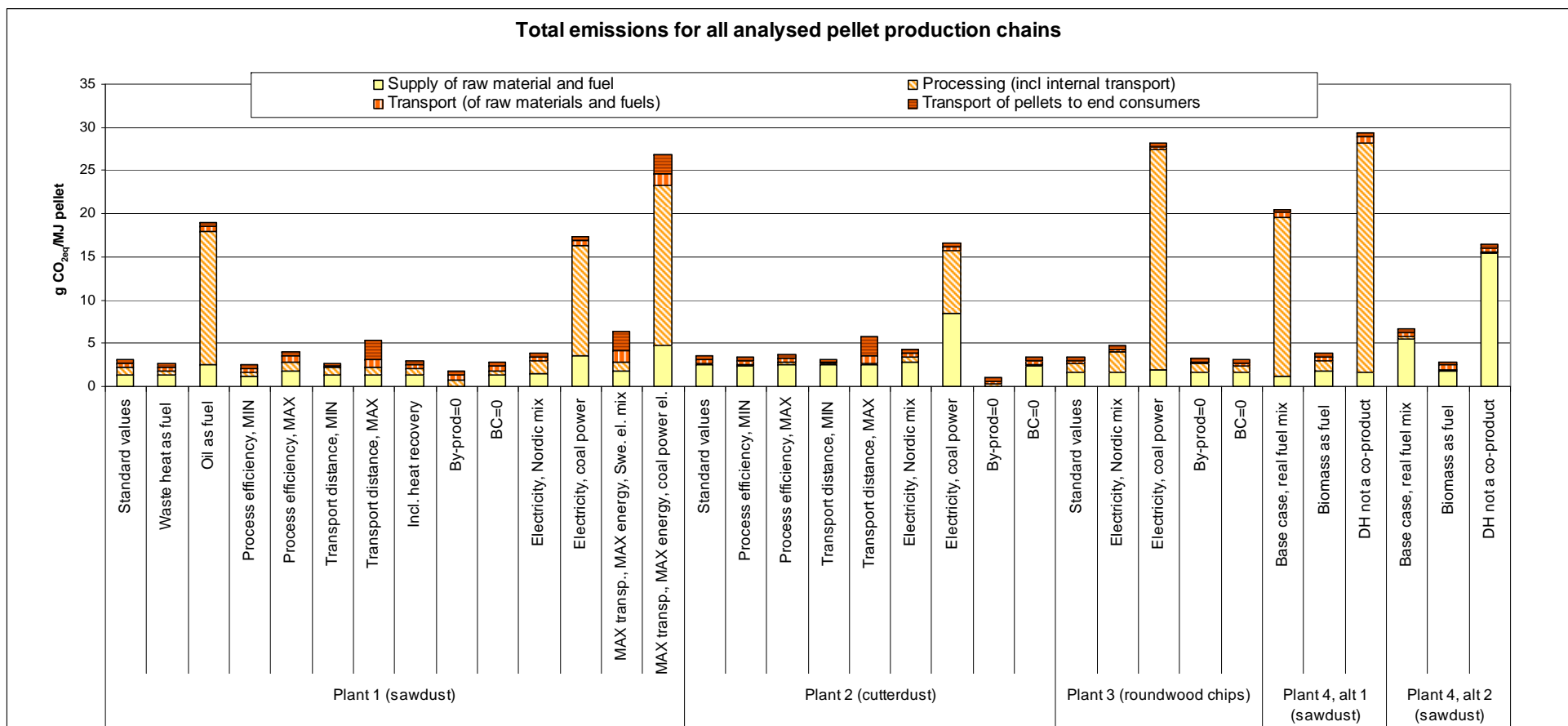
Figure 5 Summary of results for the different pellet production chains analysed. Plant 1-3 indicate production in stand-alone pellet plants. Plant 4 is production in a pellet plant integrated with a CHP plant (Hedensbyn) where alt 1) it is regarded as a poly-generation plant, and alt 2) the pellet plant and the CHP are regarded as separate plants. The following assumptions are used, if not otherwise stated: Swedish electricity mix; typical values for process efficiency (energy) and transport distances; emissions from production of saw mill by-products and biomass combustion are accounted for; biomass used for drying in Plant 1 and Plant 3; for Plant 4 the fuel mix in the CHP is 26% peat and 74% biomass and district heating is regarded as a co-product. Explanations: By-prod=0 when emissions from saw mill by-products are taken as zero; BC=0 when all emissions from biomass combustion is taken as zero. DH means district heating.
