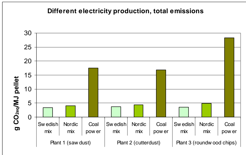
Figure 3 Total emissions for pellet production in stand-alone plants assuming different emission intensity for purchased electricity. Including end use in large scale heating plant.
