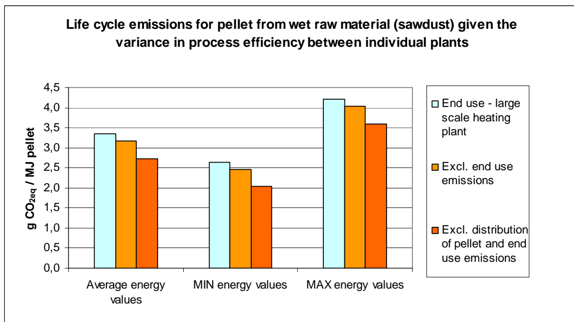
Figure 1 Emissions given the variance in process efficiency between individual plants where pellets is produced from raw sawdust and biomass is used for drying. Typical transport distances are assumed.
