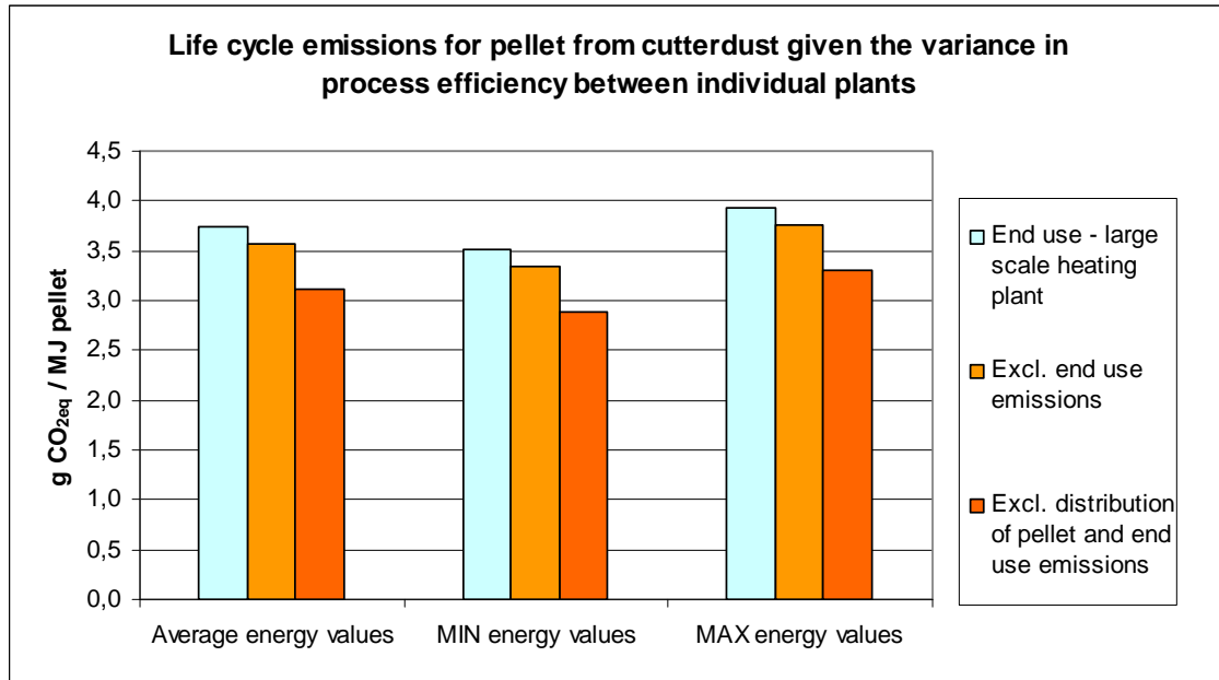
Figure 2 Emissions given the variance in process efficiency between individual plants where pellets is produced from dry materials (cutterdust) and biomass is used for drying. Typical transport distances are assumed.
