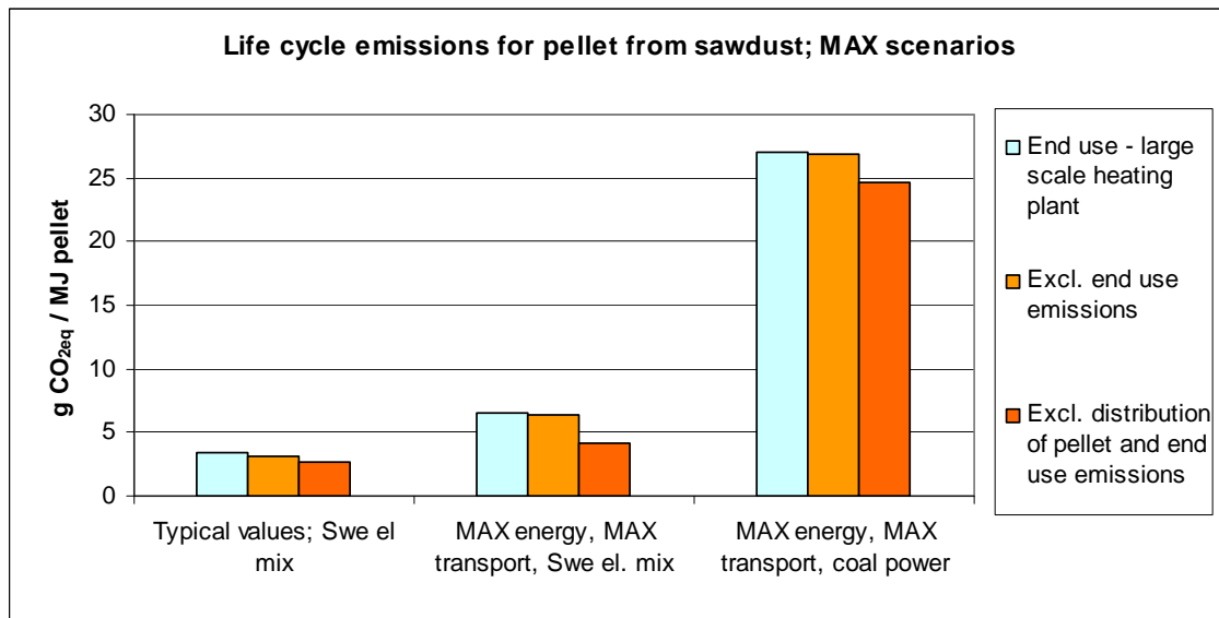
Figure 4 MAX scenarios for pellet production from sawdust in a stand-alone plant (Plant 1). For MAX energy is the maximum value for use of energy in investigated pellet plants used (i.e. low efficiency) and for MAX transport are the maximum transport distances of raw materials, fuels and pellets used. Two different emission intensity for purchased electricity.
